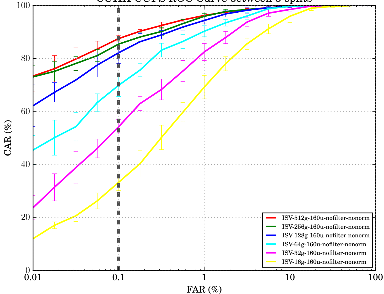
CUHK-CUFS ROC Curve between 5 splits
