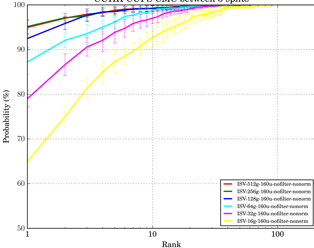
CUHK-CUFS CMC between 5 splits
